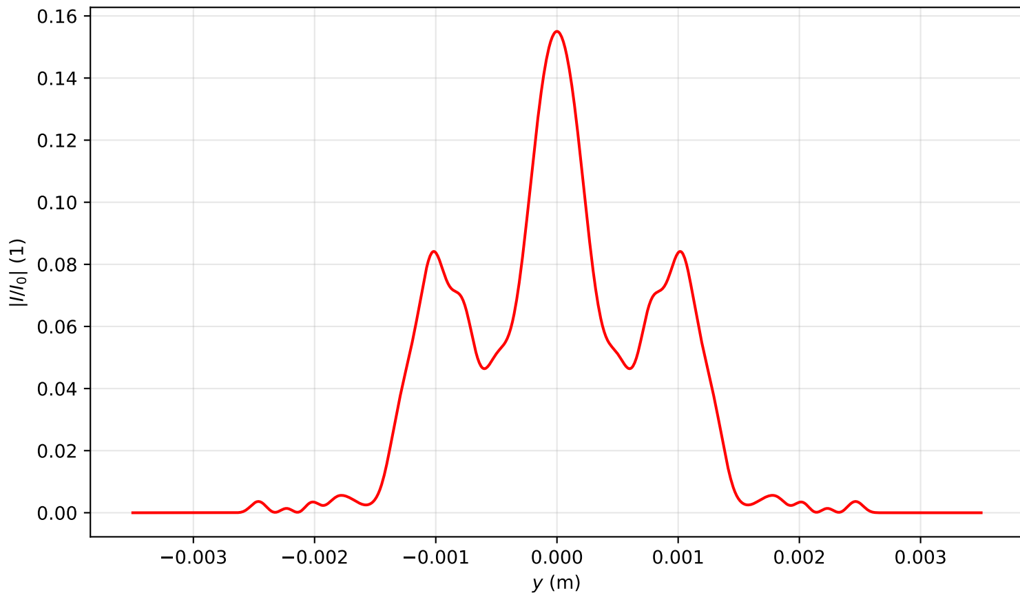
Intensity profile I(x=0, y, z=2.627)/I_0 , P_{in}=6.0P_{cr} , artificial time
